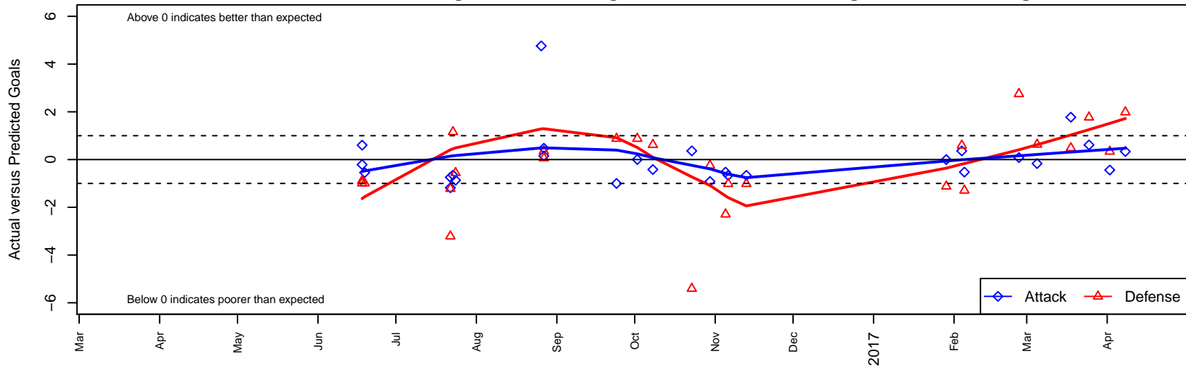
Cascade FC Green G02 Dots are actual minus expected GF (blue circles) and GA (red triangles). Blue line is smoothed change in attack strength. Red is smoothed change in defense strength.
